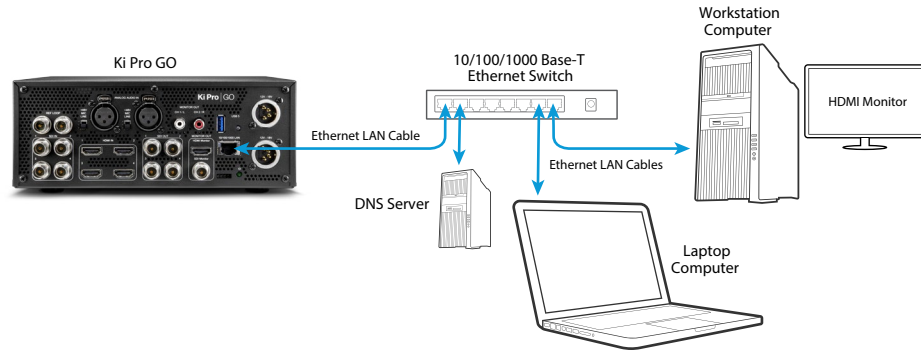
Figure 9. Ki Pro GO LAN Connection Example using a LAN
