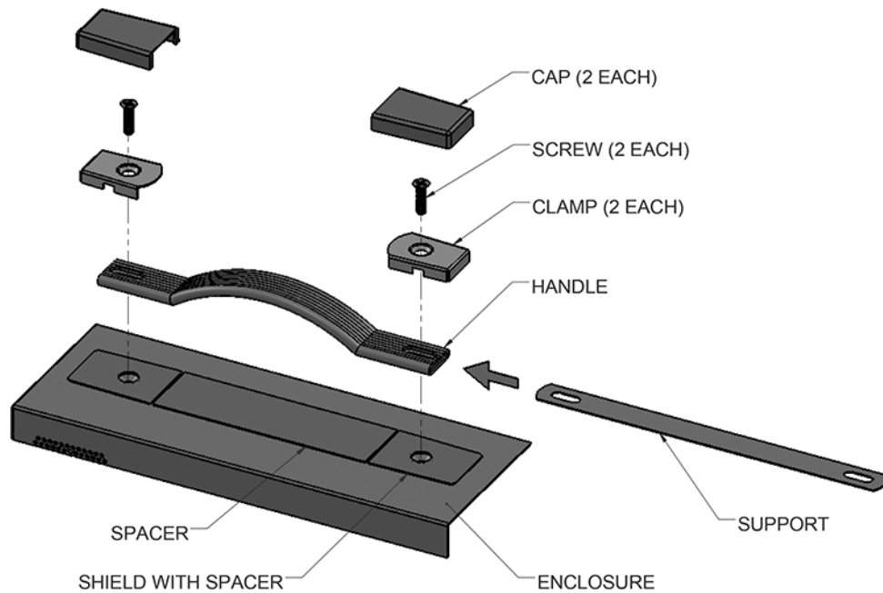
Figure 5. Ki Pro GO Handle Assembly
