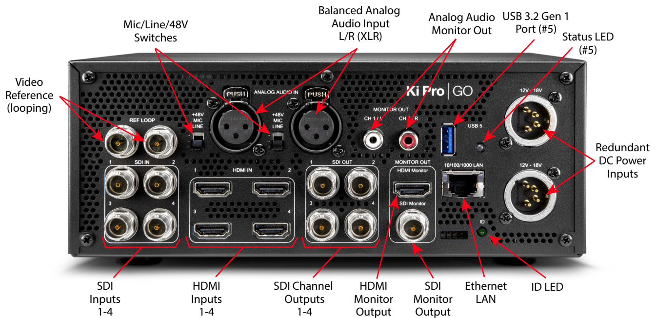
Figure 3. Ki Pro GO Rear Panel
