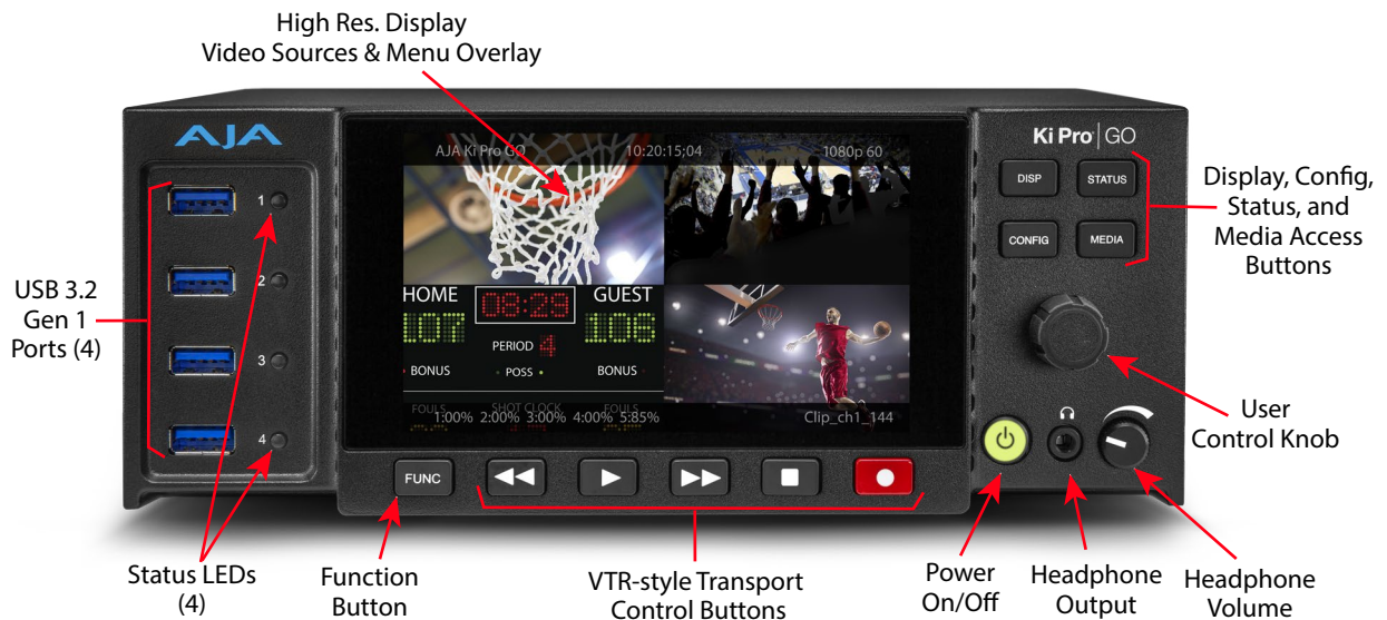
Figure 1. Ki Pro GO Front Panel
