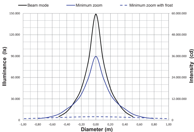
Mythos - Illuminance Distribution at distance = 20m
