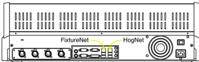
Figure 3.9. HogNet and FixturerNet Connections on back panel of Road Hog 4 Console
