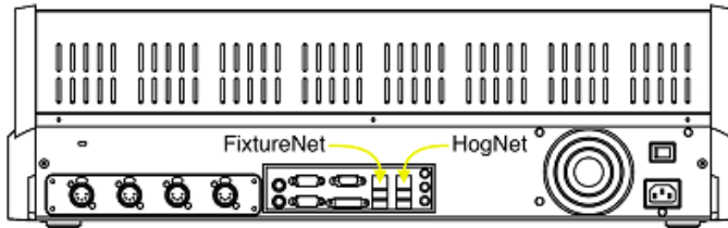
Figure 35.1. Back panel of Road Hog 4 Console
