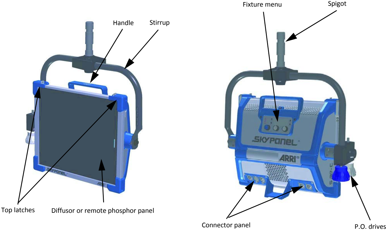
Figure 2: Front and back view, P.O. version (the figure shows the S30)
