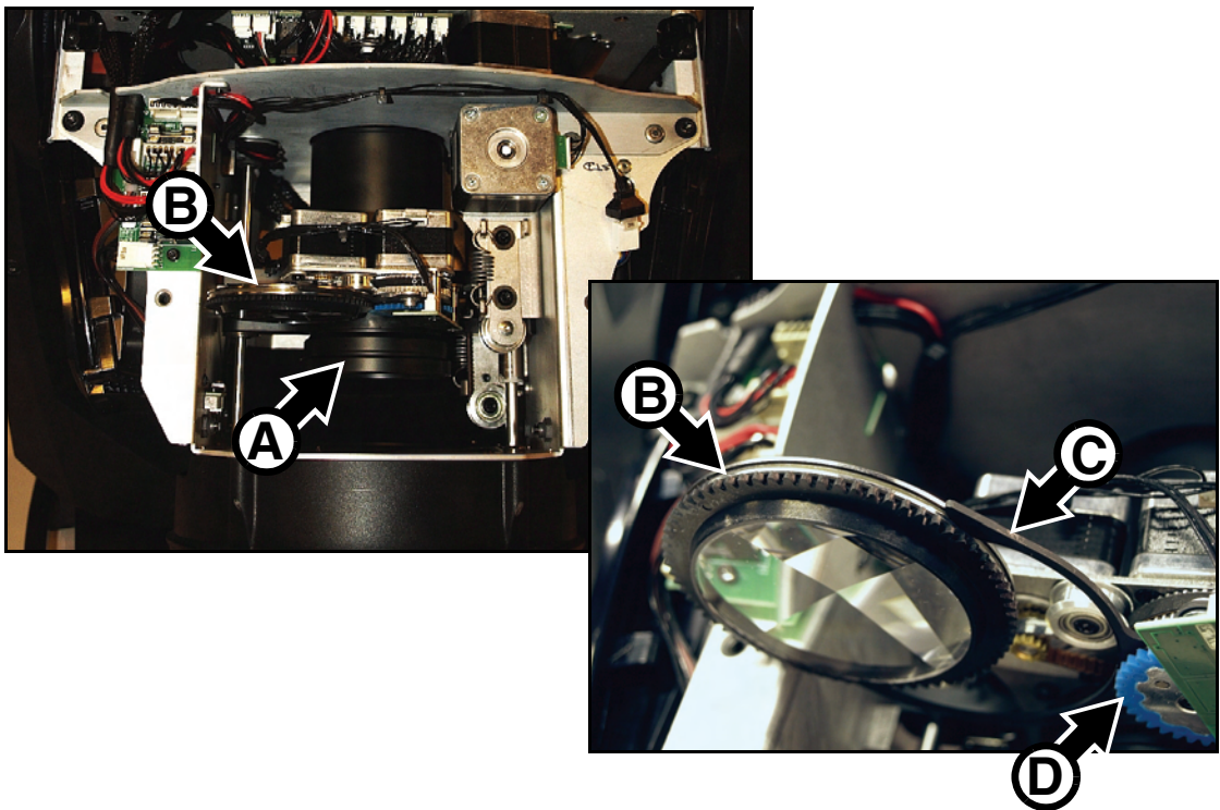
Figure 16: Prism removal and installation
