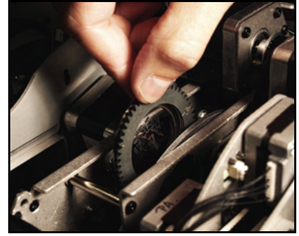
Figure 19: Gobo removal
