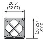
END VIEW
